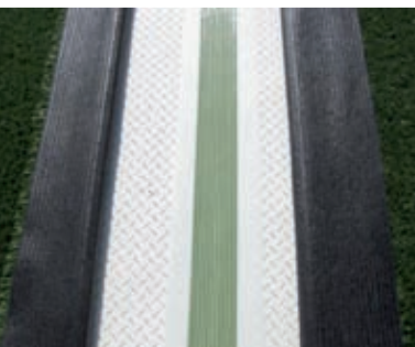
10 | Gluing of turf, adhesive coated fleece and turned down turf edges
