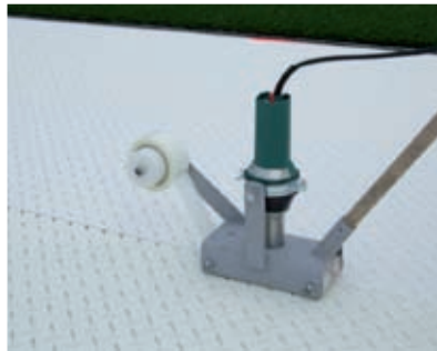
4 | Mobile welding machine with adhesive tape to weld roll joints
