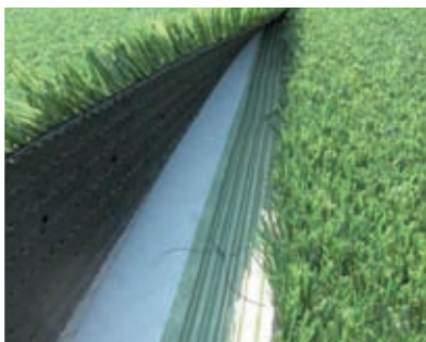
11 | Lamination of turf with fleece and 2-component adhesive
