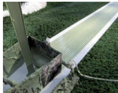
9 | Lamination of turf with fleece and 2-component adhesive
